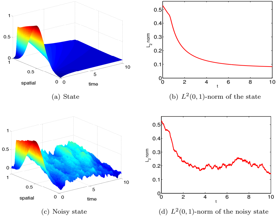
FIG. 5. Uncontrolled solutions for Example 3
