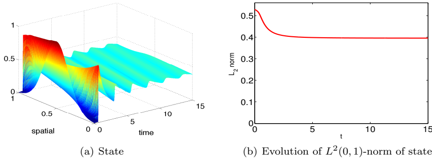
FIG. 1. Uncontrolled solution for Example 1
